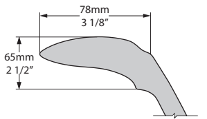
Rim Detail
