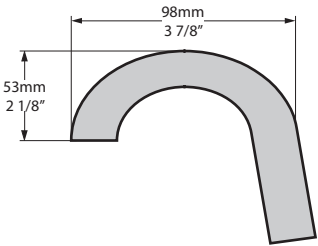
Rim Detail
