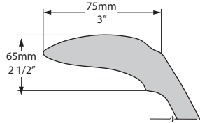
Rim Detail
