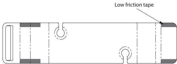
Underside View
