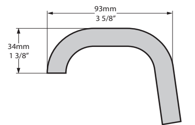
Rim Detail
