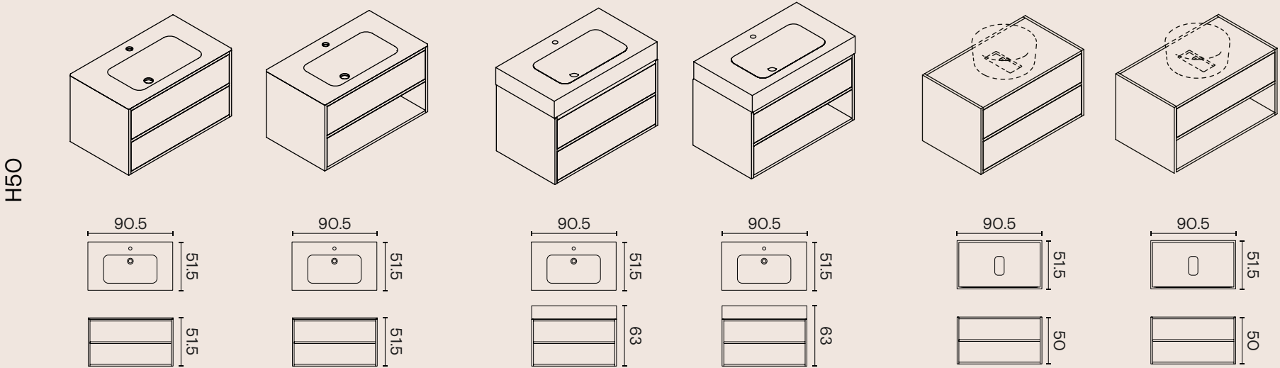
With integrated basin 90 top
